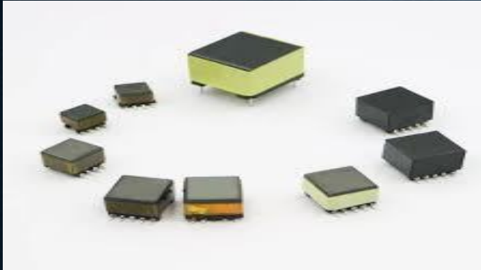
EP TFR (EP5 – EP17) Ae- 3 to 34 , Power -5W to 50W
